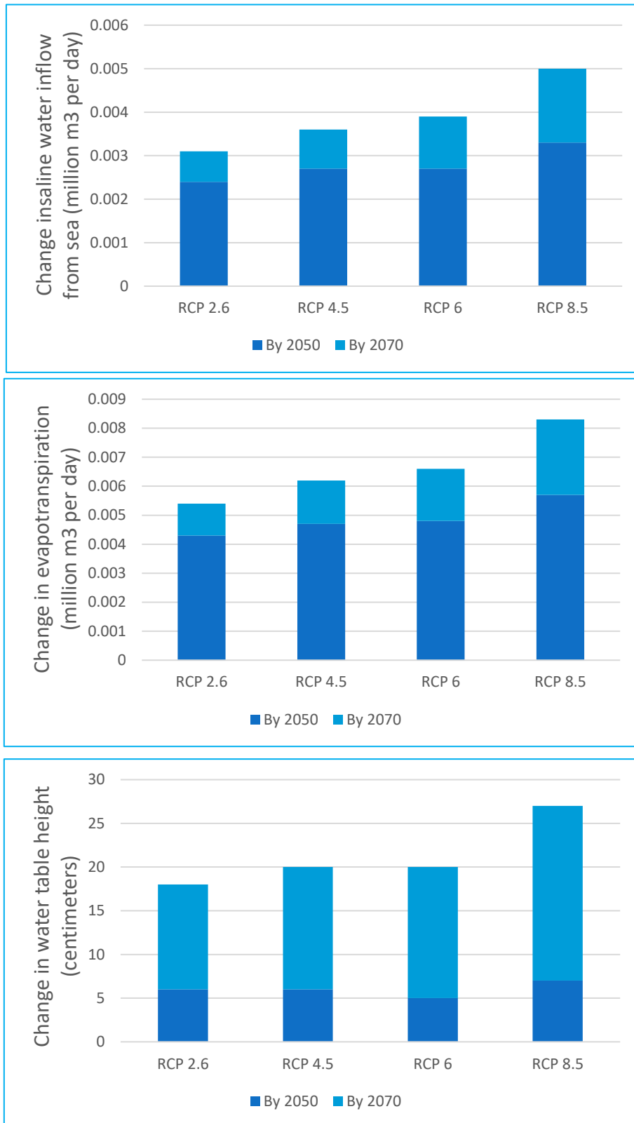
Figure 15: Impacts of sea level intrusion in the Samail lower catchment aquifer near Muscat by 2050 and 2070 (Al Maktoumi et al, 2015)
