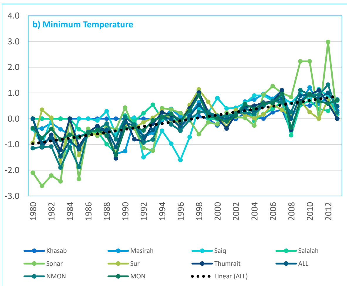
Figure 4: Maximum (a) and Minimum (b) Temperature trends in Oman (AL Maskari et Al, 2015)
