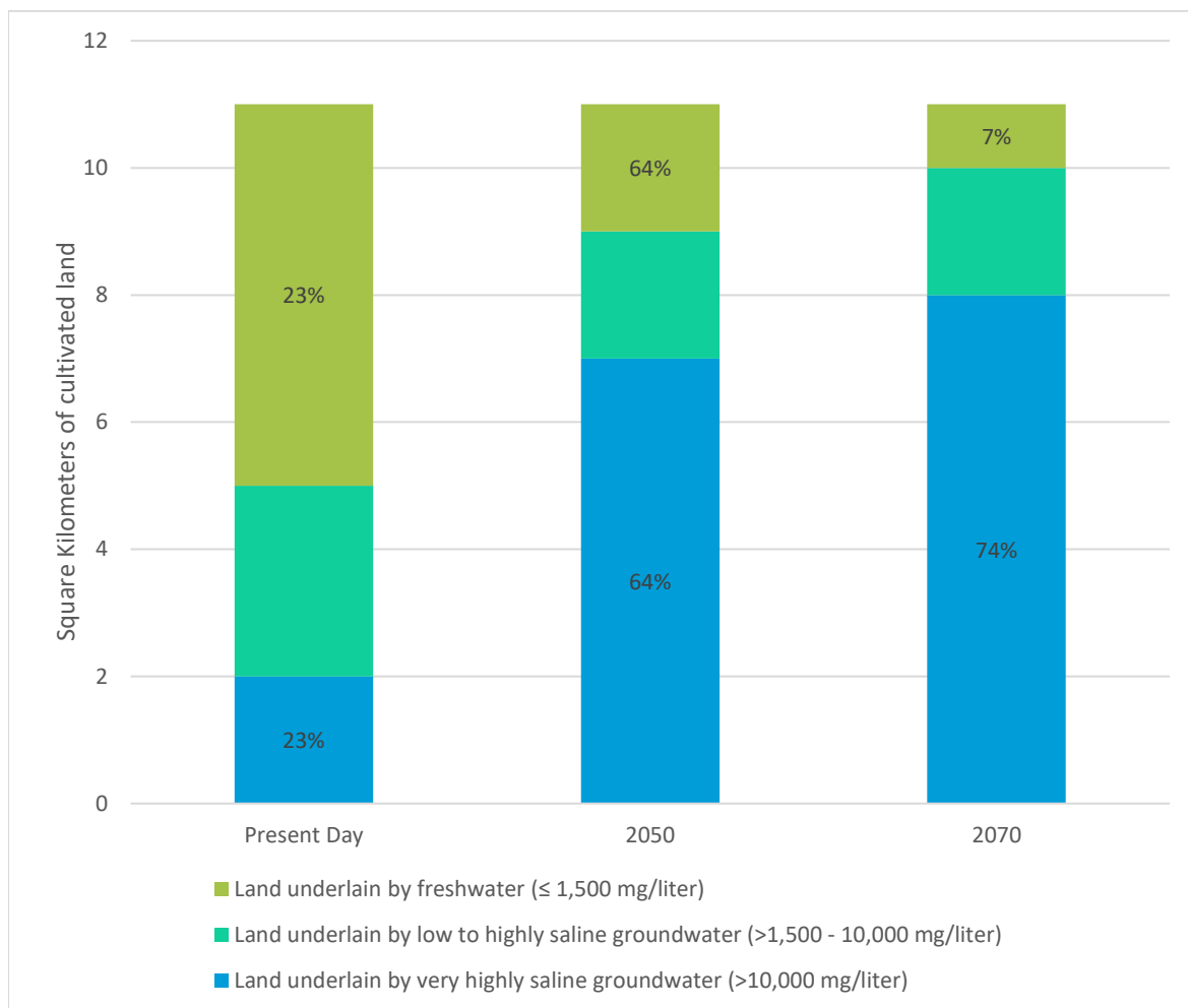
Figure 21: Loss of cultivatable land due to groundwater quality deterioration from sea level rise in Al Batinah (Zekri, 2015)
