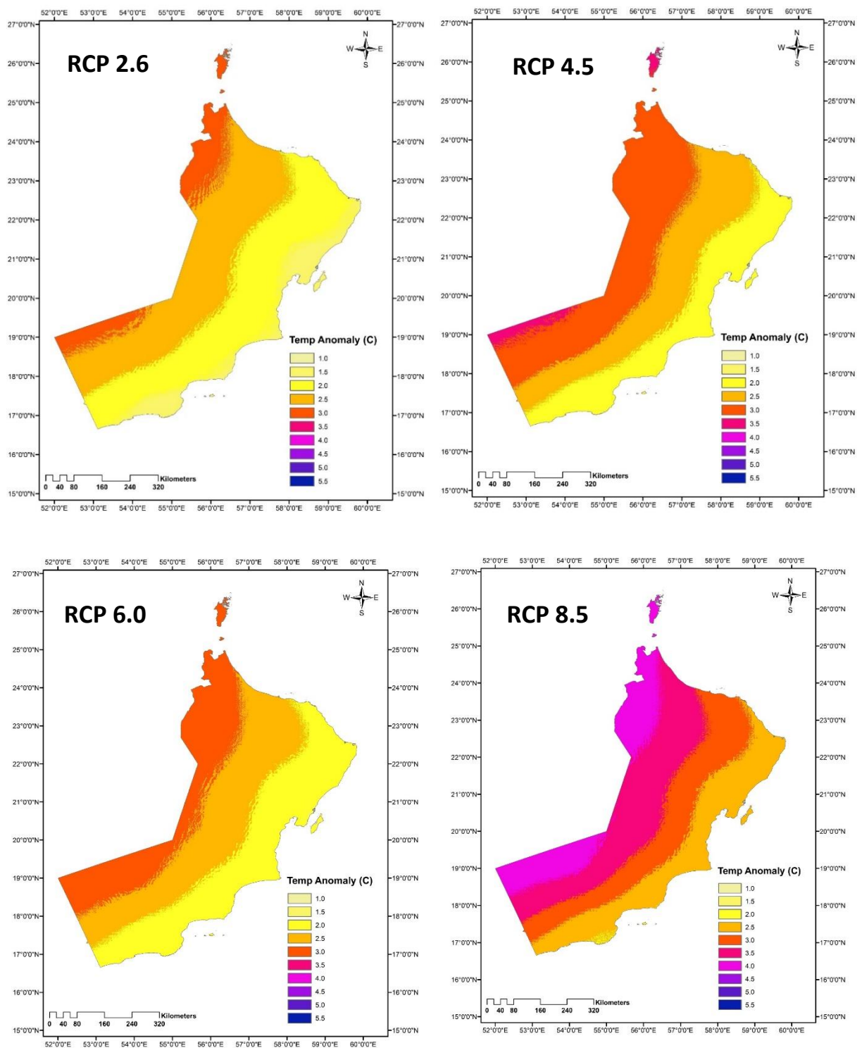
Figure 6: Maximum temperature change by 2041-2060 relative to historical period, for all RCPs (Al Maskari et al, 2015)
