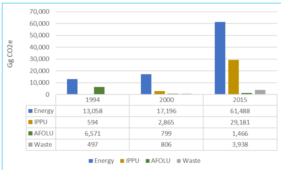
Figure 32: Trends in total GHG emissions by gas type and emitting sector (SoO, 2013 for 1994; Charabi, 2017 for 2000 and 2015)
