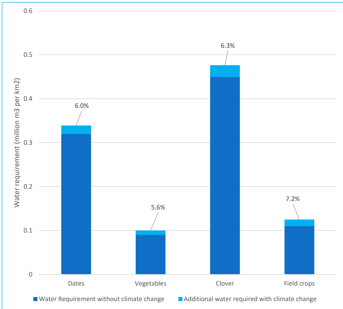
Figure 22: Impact of evapotranspiration on crop water requirements in Oman (Zekri, 2015)
