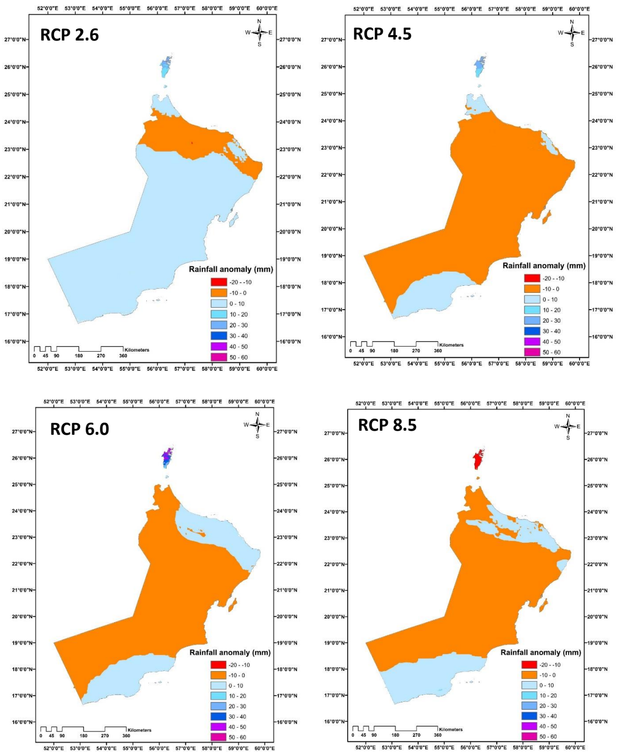
Figure 10: Average annual rainfall change by 2041-2060 relative to historical period, for all RCPs (Al Maskari et al, 2015)
